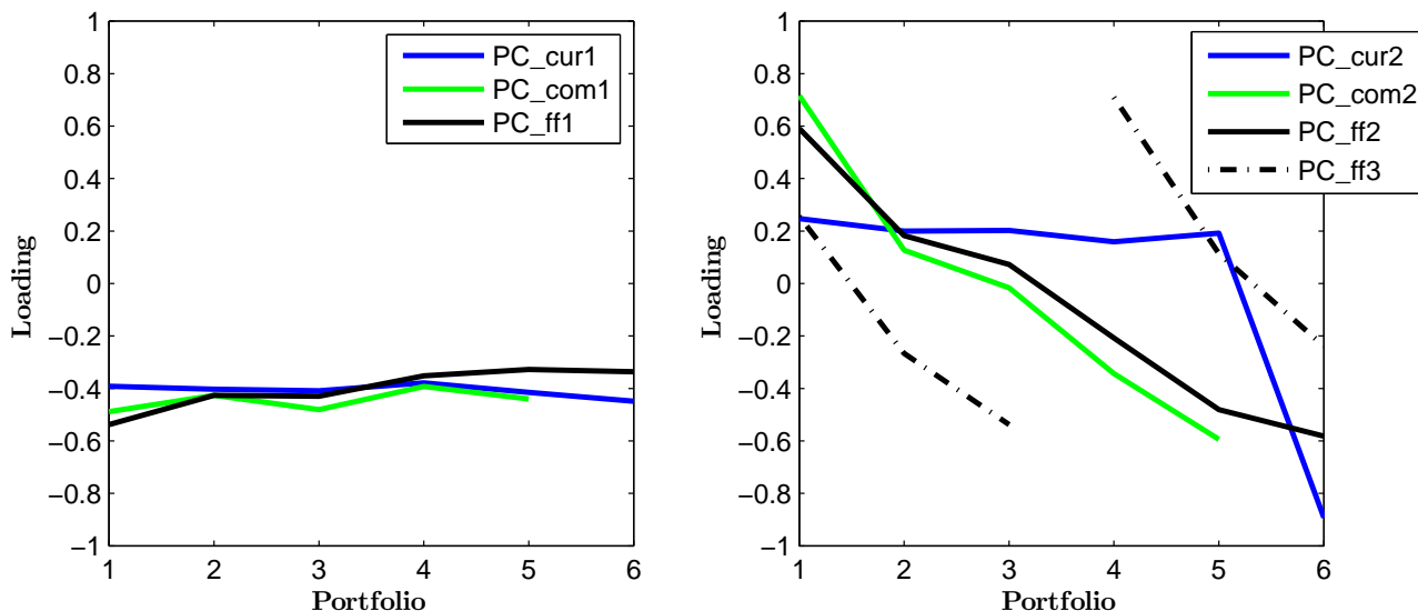
Figure 14: PCA Loadings: Currencies, Equities, and Commodities
