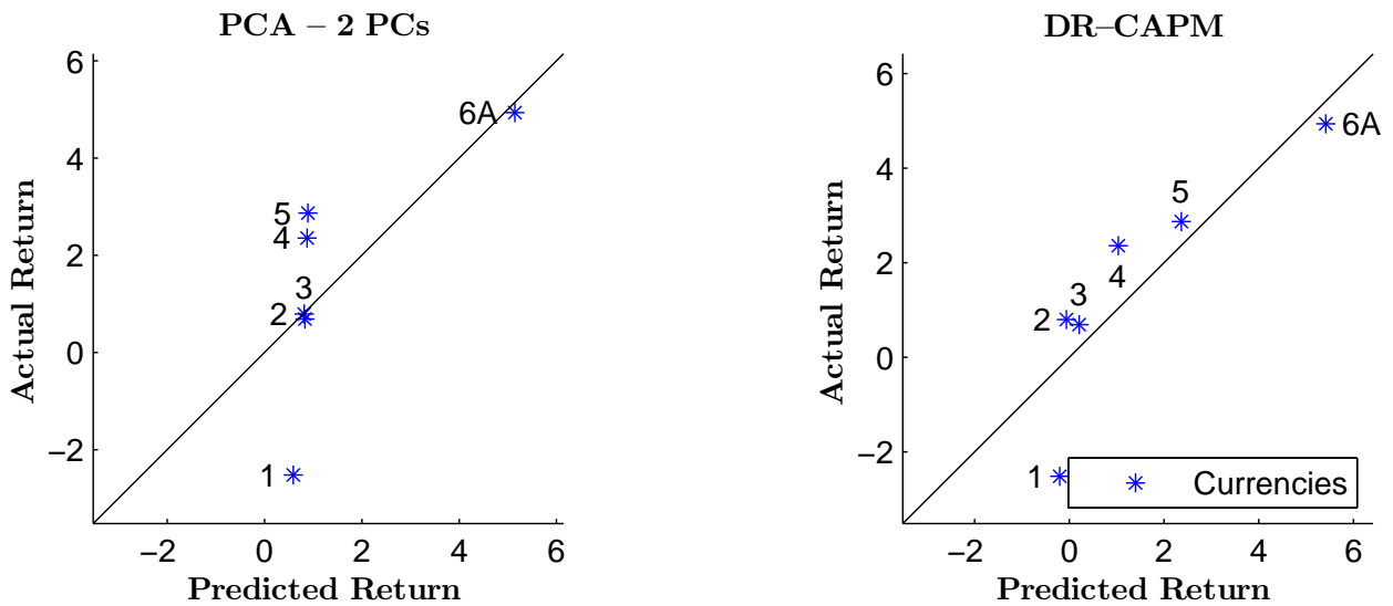
Figure 11: Model Performance: PCA Currencies
