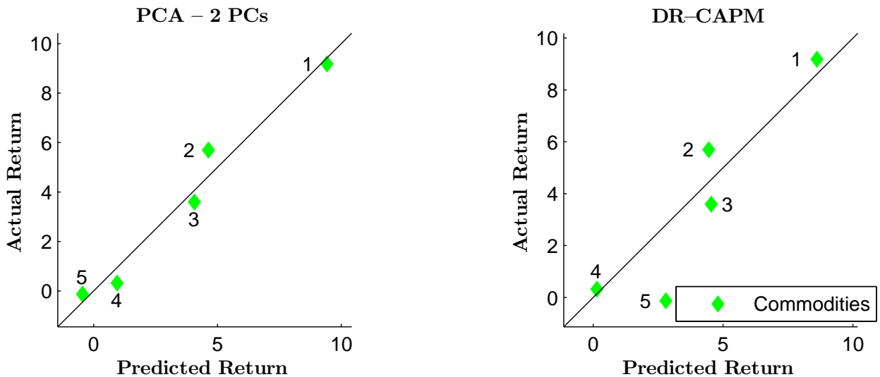
Figure 13: Model Performance: PCA Commodities
