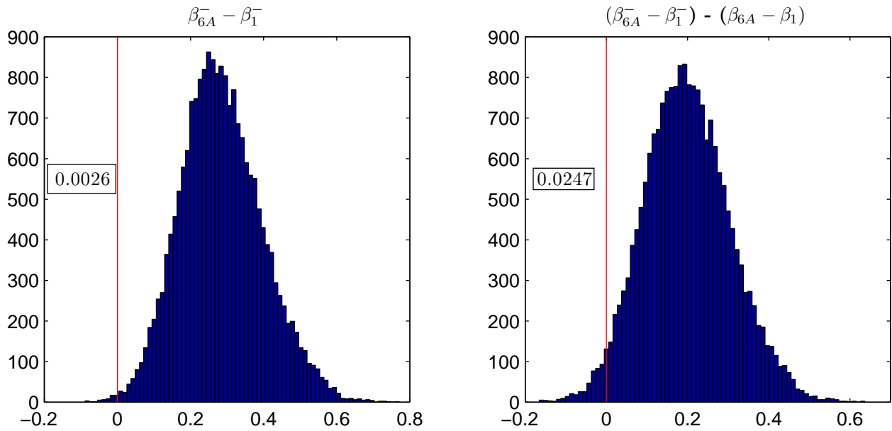
Figure 10: Bootstrapped Distribution: Relative Downstate Betas
