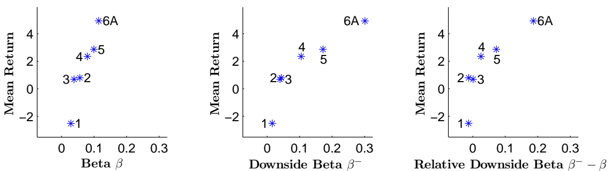
Figure 3: Risk-Return Relations: Currencies
