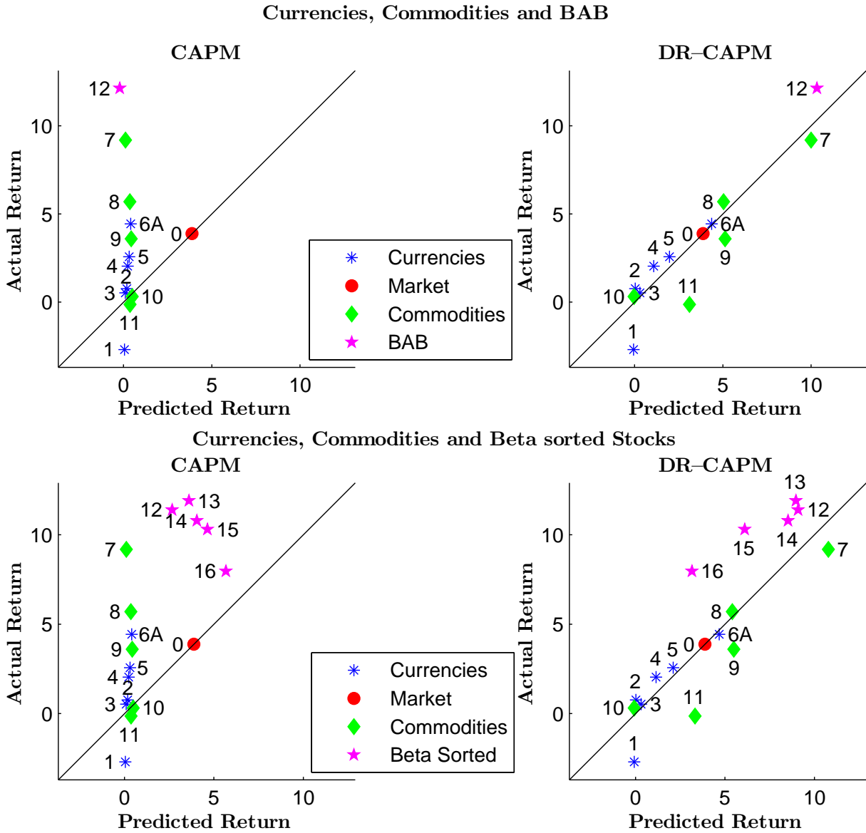
Figure 9: Model Performance: Currencies, Commodities and Beta sorted Stocks
