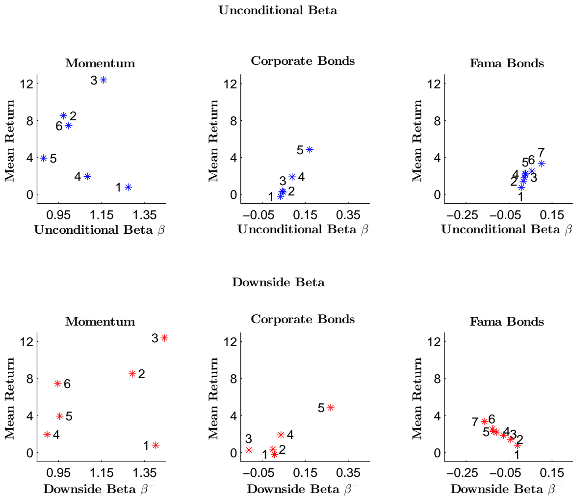
Figure 15: Risk-Return Relations: T-Bills, Equity Momentum, Corporate Bonds
