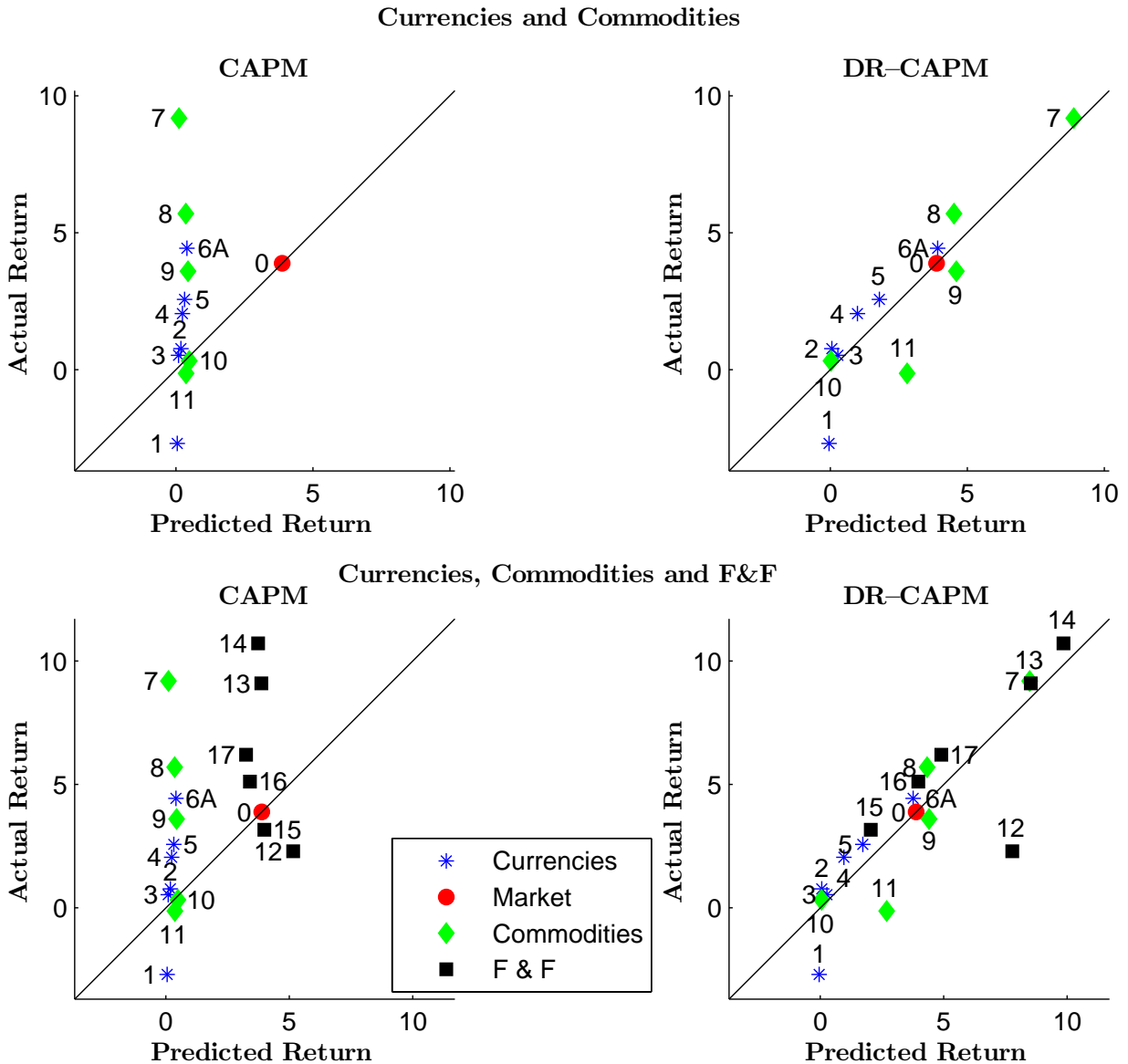
Figure 7: Model Performance: Currencies and Commodities
