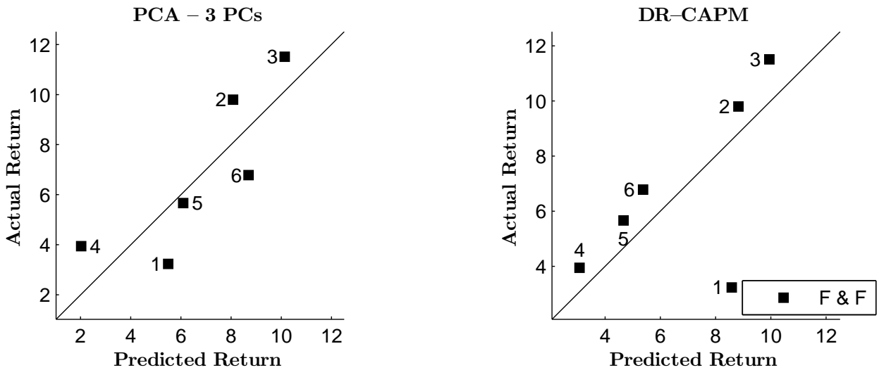
Figure 12: Model Performance: PCA Stocks
