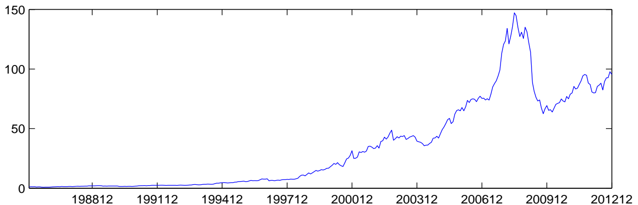
Plot C: Wealth process of long-short strategy
