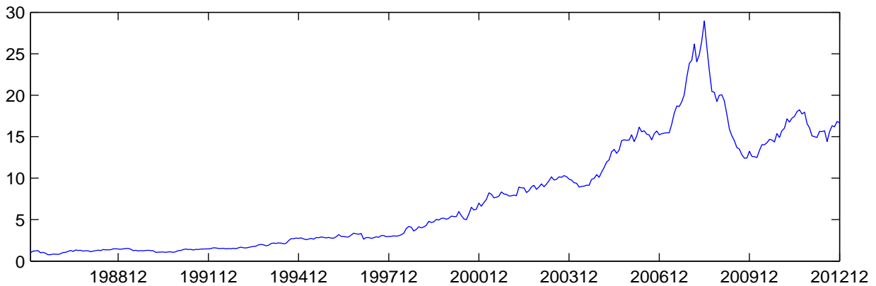
Plot A: Wealth process of long leg of strategy
