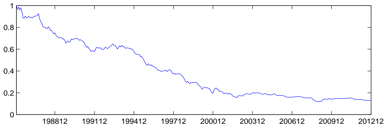
Plot B: Wealth process of short leg of strategy
