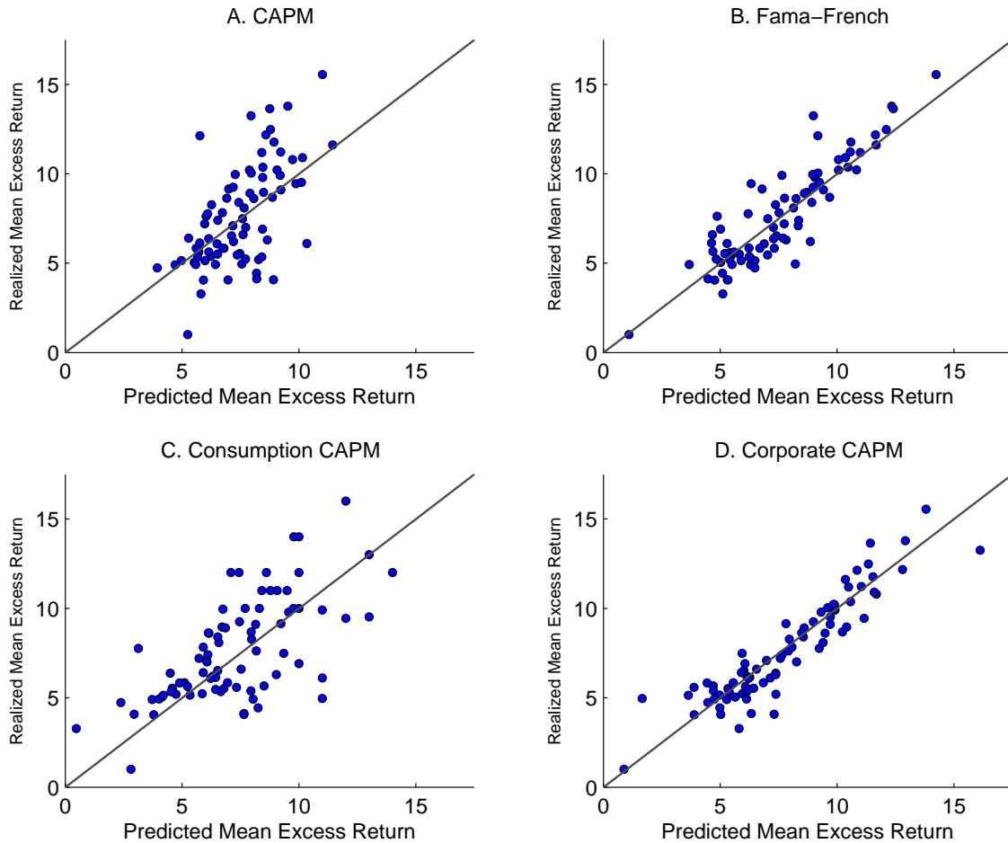
Figure 6. Predicted vs Realized Excess Returns: Comparison Among Models.
